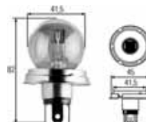
Two-filament bulb 40/45watt, 6 volt!
