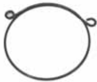
Fastening spring for rubber grease cap for pin bearing, front axle, for 111CV, measure: 63x69x3mm, Or.no.: 426623
