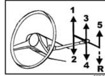
R16, label for the gear shift (is appropriate at the windshield). Suitable for Renault R16. 5 speed gearbox.
